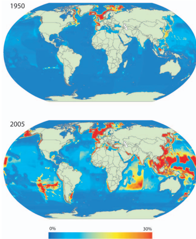
Figure 1. Primary production required (PPR) to sustain global marine fisheries landings expressed as percentage of local primary production (PP). Estimates of PPR, PP and PPR/PP computed per 0.5° latitude/longitude ocean cells. PPR estimates based on the Sea Around Us catch database ( www.seaaroundus.org ) and PP estimates derived from SeaWiFS's global ocean colour satellite data. The maps represent total annual landings for 1950 (top) and 2005 (bottom). Note that PP estimates are static and derived from the synoptic observation for 1998. doi:10.1371/journal.pone.0015143.g001
