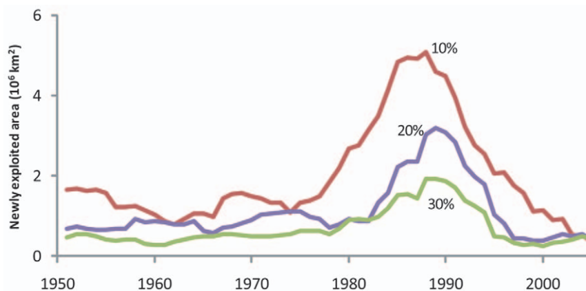
Figure 2. Time series of areas newly exploited by marine fisheries (1950–2005), expressed in km 2 . Newly exploited areas defined as regions where primary production required (PPR) to sustain reported fisheries landings exceeds the threshold percentage of local primary production (PP). Results based on three exploitation thresholds (10%, 20% and 30%) are presented. doi:10.1371/journal.pone.0015143.g002
