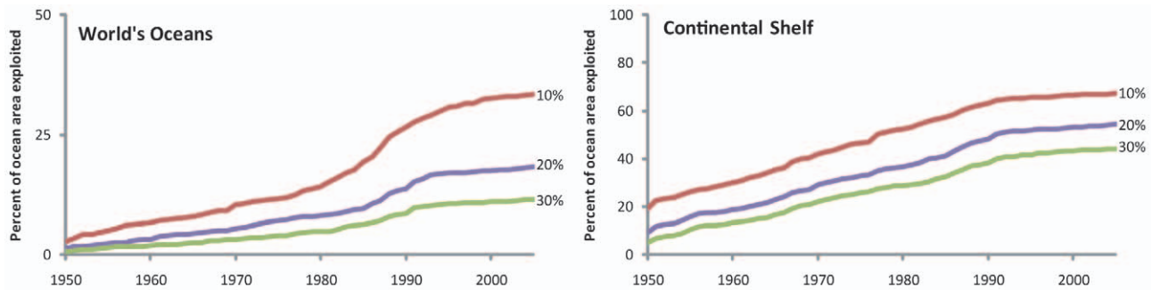
Figure 3. Time series of areas exploited by marine fisheries (1950–2005) expressed as a percentage of the total ocean area. 'Area exploited' defined as regions where primary production required (PPR) to sustain reported fisheries landings exceeds the threshold percentage of local primary production (PP). Results based on three exploitation thresholds (10%, 20% and 30%), and for all marine areas (left) and continental shelf areas (i.e., up to 200 m in depth, right) are presented.
